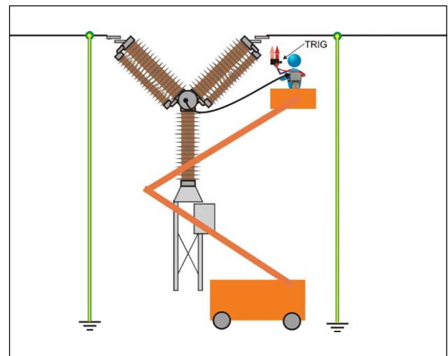
Measurement on CB with both sides grounded, DualGround.
